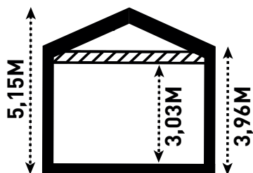
CUTTING PLAN
